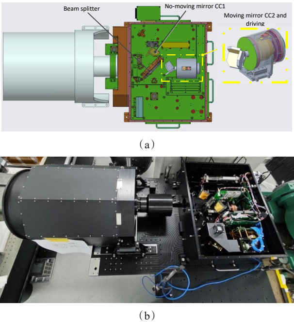
Fig. 5 Instrument structure of the interferometer based on the angular mirror translation system 图5 基于角镜平动式干涉系统的仪器结构图
