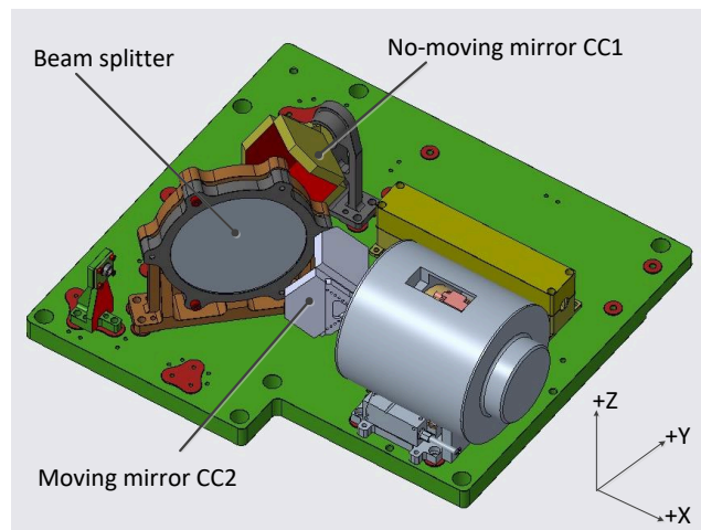
Fig. 3 Model of the interferometer
