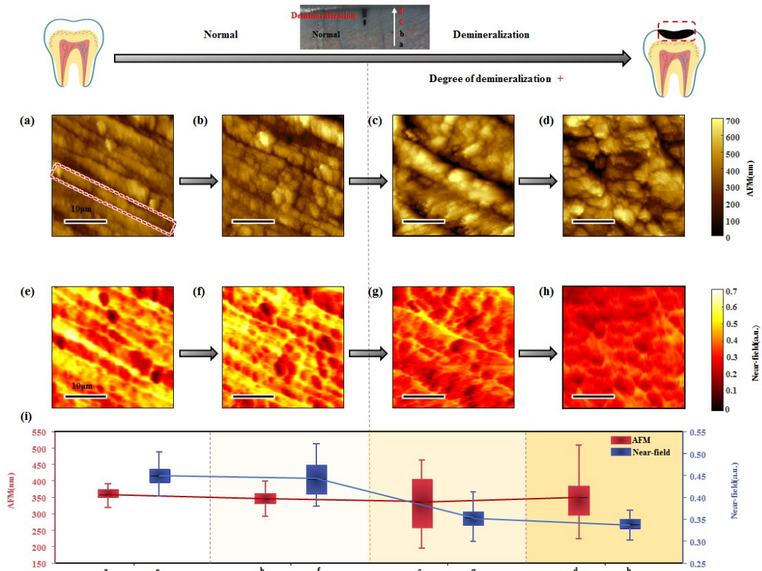
Figure 3 (a)-(d) AFM results. (e)-(h) Near-field imaging results. (i) The boxplot of AFM and near-field data in each region. The black line in each box represents the mean value which is connected to form the mean value line.
