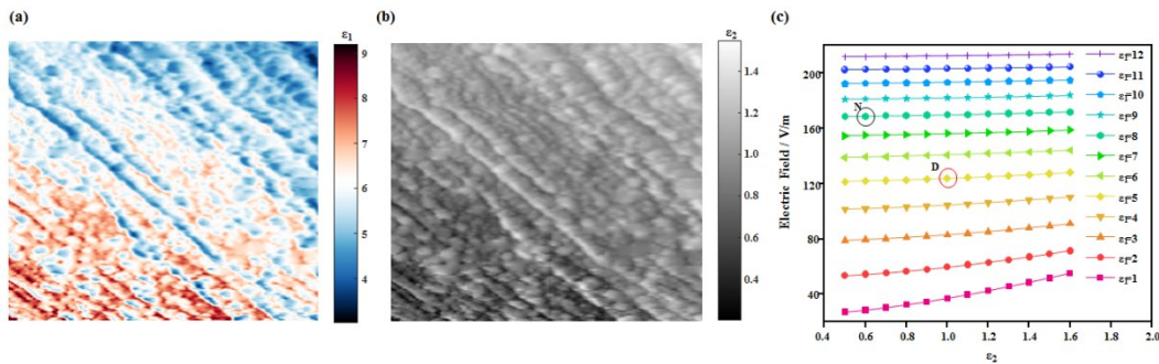
Figure2 (a) The real part of the dielectric constant of enamel. (b) The imaginary part of the dielectric constant of enamel. (c) Influence of \epsilon_1 and \epsilon_2 changes on near-field signal (The black circle represents normal enamel and the red represents demineralized enamel).
