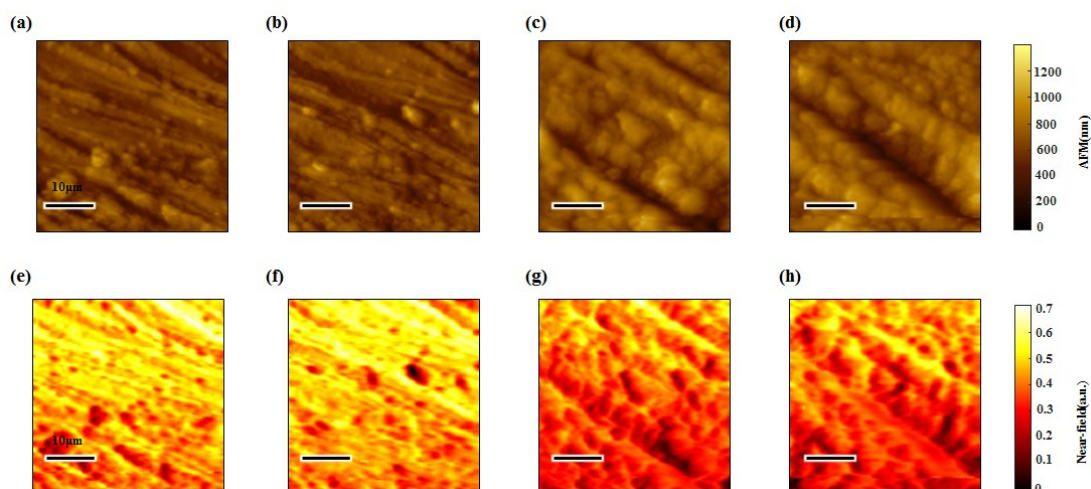
Figure4 (a)-(b) AFM results in normal enamel. (c)-(d) AFM results in demineralized enamel. (e)-(f) Near-field imaging results in normal enamel. (g)-(h) Near-field imaging results in demineralized enamel.
