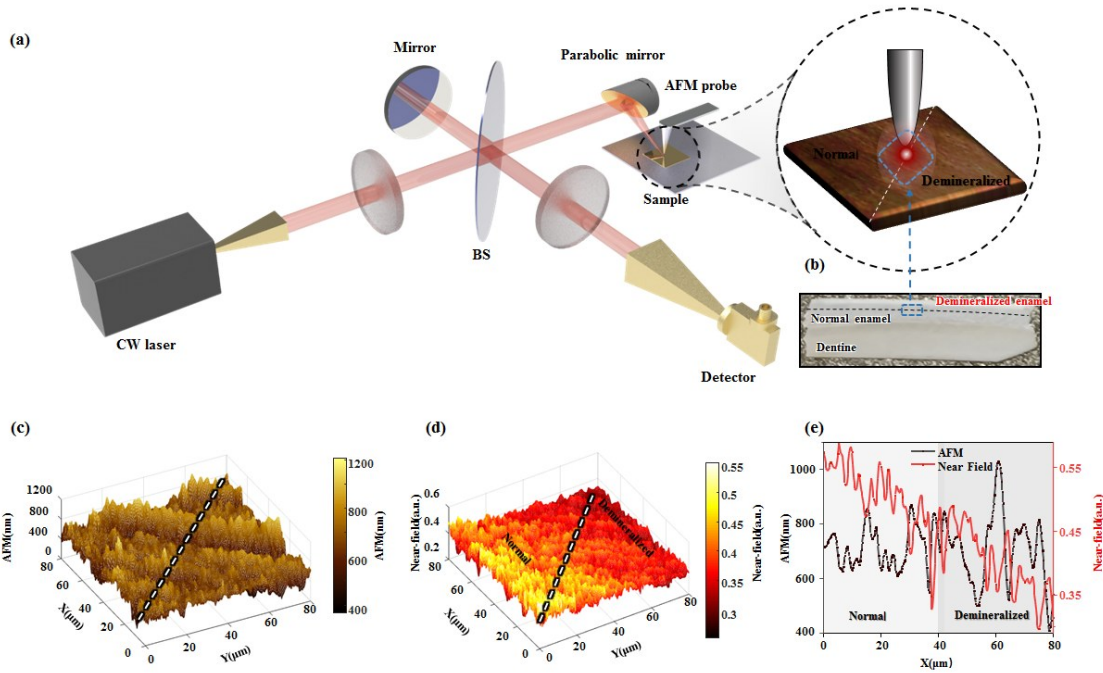
Figure1 (a) Schematic illustration of the CW THz-SNOM setup. (b) Photo of the tooth slice (the area highlighted by the blue curve is the scanning range). (c) AFM results. (d) Near-field imaging results. (e) AFM and near-field signals along the dashed line.
