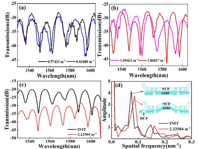
Fig. 9 (a) Transmission spectrum of the MTP-MZI with HCF at curvature of 0.57433 m -1 , 0.8348 m -1 and (b) 1.09462 m -1 , 1.86817 m -1 , respectively; (c) The transmission spectrum of the MTP-MZI with HCF at curvature of 2.22504 m -1 and the straight MTP-MZI without HCF; (d) The corresponding spatial spectra
