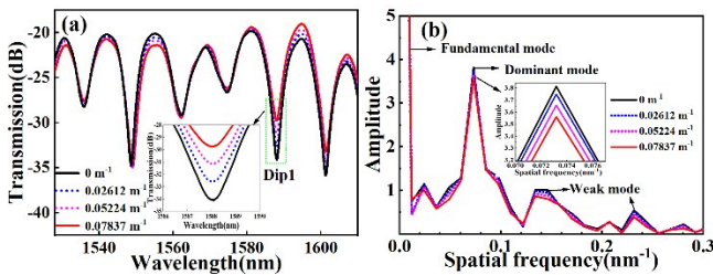
Fig. 6 (a) The transmission spectra of MTP-MZI with variation curvatures; (b) The corresponding spatial frequency spectrum
