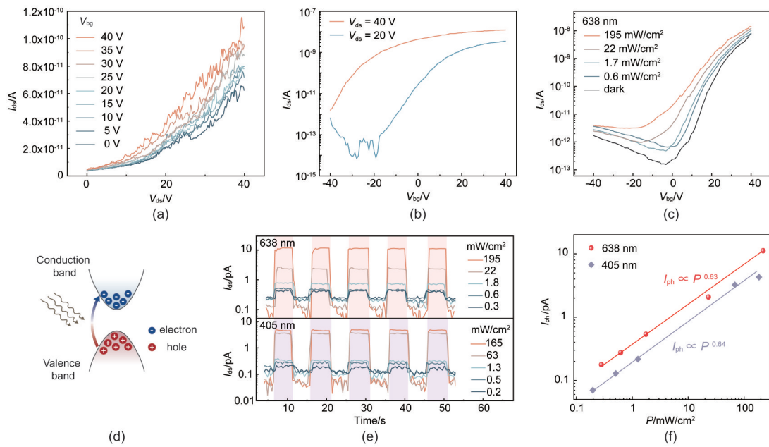
Fig. 2 Electrical and photoresponse of Y6-10 phototransistor with thickness of 106 nm: (a) output characteristic curve at different bias gate voltages; (b) transfer characteristic curves under different drain-source voltages; (c) transfer characteristic curves at different power densities of 638 nm, V_{ds} = 40 V; (d) schematic diagram of photoresponse band of Y6-10 crystal; (e) photoresponse of Y6-10 transistor at different power densities of incident light at 638 nm and 405 nm, V_{ds} = 40 V; (f) the photocurrent of 638 nm and 405 nm irradiation as a function of the incident light power
