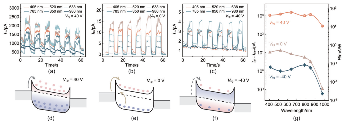
Fig. 3 Photoresponse of Y6-10 under different gate voltages: (a–c) the photoresponses for light from 400 nm to 1 000 nm under different gate voltages of 40 V (a), 0 V (b), and -40 V (c), when P = 10 mW/cm 2 and V_{ds} = 40 V; (d–f) schematic of the band diagrams under gate voltage of 40 V (d), 0 V (e), and -40 V (f); (g) the spectral response of the Y6-10 phototransistor at different gate voltages
