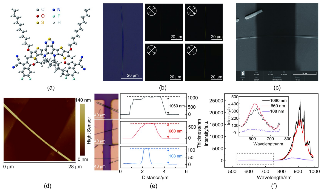
Fig. 1 Y6-10 organic semiconductor materials and characterization: (a) Y6-10 atomic structure with high conjugation; (b) polarization optical microscope image of Y6-10 single crystal (scale: 20 \mu m), the arrows indicate the polarization of the incident and collected light; (c) field emission scanning electron microscopy (SEM) images of Y6-10 organic transistors; (d) atomic force microscopy (AFM) images of Y6-10 organic transistors; (e) thickness profile of Y6-10 organic materials and their corresponding optical images; (f) photoluminescence (PL) spectral properties of Y6-10 crystals with 1 060 nm, 660 nm and 106 nm thickness
