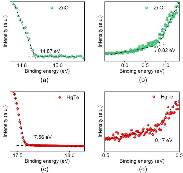
Fig. 2 The UPS of HgTe QDs and ZnO QDs: (a)~(b) Valence band spectrum and second electron cutoffs of ZnO; (c)~(d) Valence band spectrum and second electron cutoffs of HgTe
