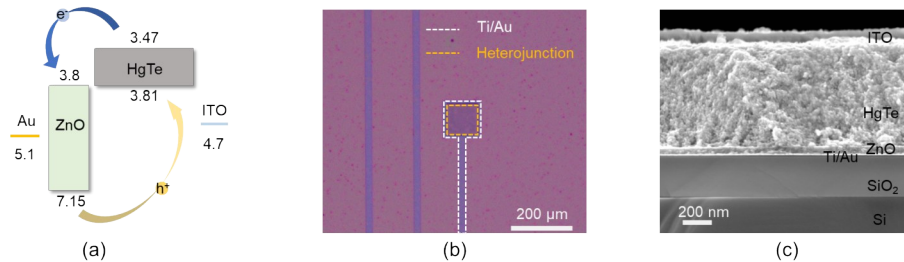
Fig. 3 The HgTe QDs/ZnO QDs heterojunction: (a) Energy band diagram of the device; (b) the optical image of device; (c) the Cross-sectional SEM image of device
