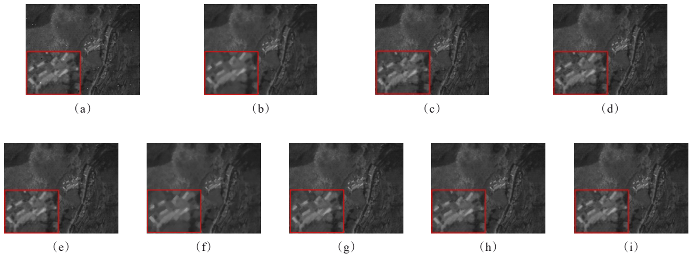
Fig. 13 Different state-of-the-art methods for denoising LWIR raw images: (a) raw image; (b) MF; (c) BdCNN; (d) HONTV-OGS; (e) \ell_0 -OGSTV; (f) DTN; (g) DCNN; (h) ALOHA; (i) Proposed
