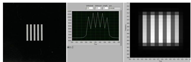
Fig. 2 (a) The square wave target; (b) MTF calibration of mid-wave infrared camera using a square wave target
