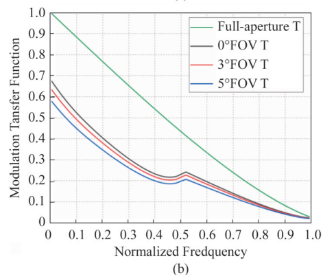
Fig. 9 The degradation of MTF, (a) different incident wavelengths, (b) different Angle of incidence 图9 MTF变化曲线, (a)不同入射波长, (b)不同入射角
