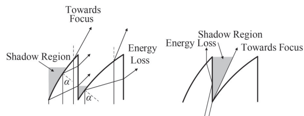
Fig. 2 Shadow effects in continuous phase structure, (a) normal incidence, (b) oblique incidence 图2 连续相位结构中阴影效应, (a) 正入射, (b) 斜入射
