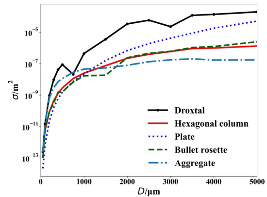
Fig. 4 Variation of backscattering cross section of ice crystals with different shapes of the maximum dimension D
