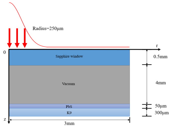
Fig. 7 Theoretical model of PbS detector irradiated by 2.79 \mu\text{m} laser
