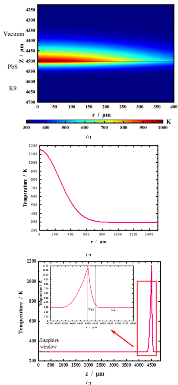
图 8 PbS 探测器的温度场分布, (a) PbS 探测器温度等值云图, (b) PbS 光敏面上的温度分布, (c) 模型轴线上的温度分布 Fig.8 Temperature distribution with laser fluence of 10 \text{ J/cm}^2 , (a) contour of temperature distribution in PbS detector, (b) temperature distribution on PbS surface, (c) temperature distribution on axis
