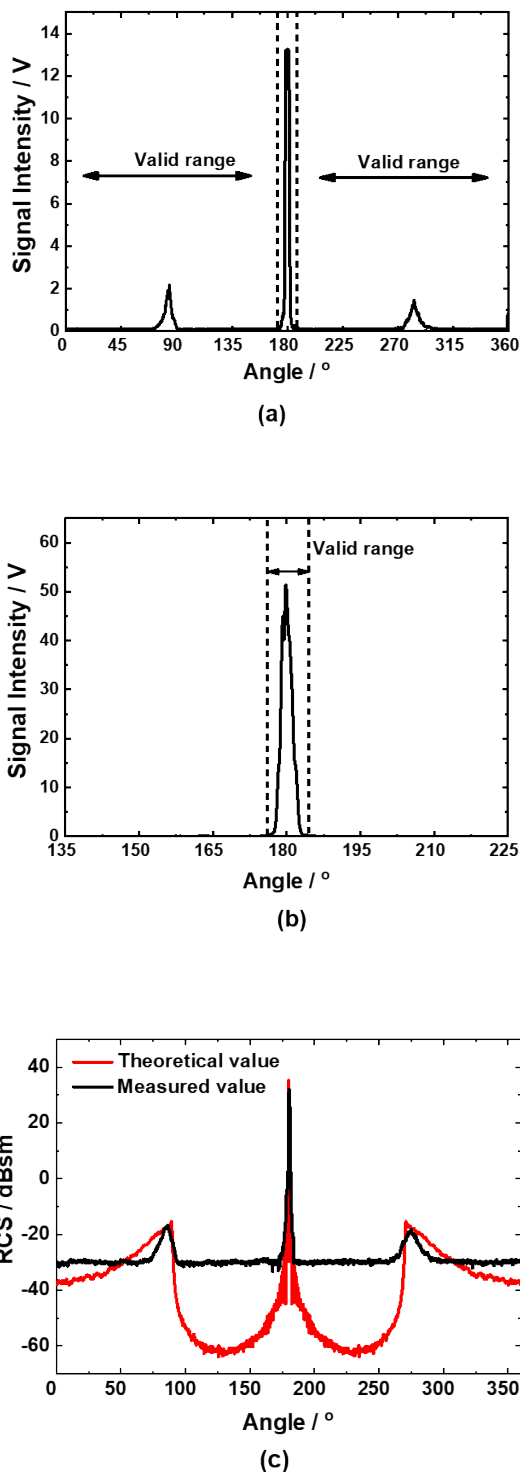
图5 弹头散射特性测量结果 (a) 球体定标散射数据, (b) 平板定标测量数据, (c) 分段处理后组合的弹头RCS结果 Fig. 5 Measurement of warhead scattering characteristics (a) Scattering signal with sphere calibration, (b) Scattering signal with plate calibration, (c) RCS results of the warhead by combining subsection processed data
