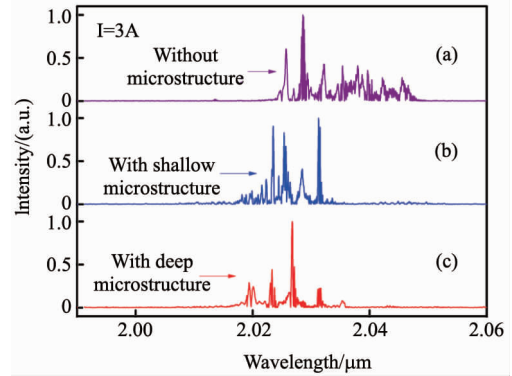
Fig. 3 Measured emission spectra of GaSb based BA lasers without (purple line), with shallow (blue line) and with deep (red line) microstructure at 3 A 图3 电流为 3 A 时,无结构,浅刻蚀微结构和深刻蚀微结构的宽脊型 GaSb 基激光器的光谱特性
