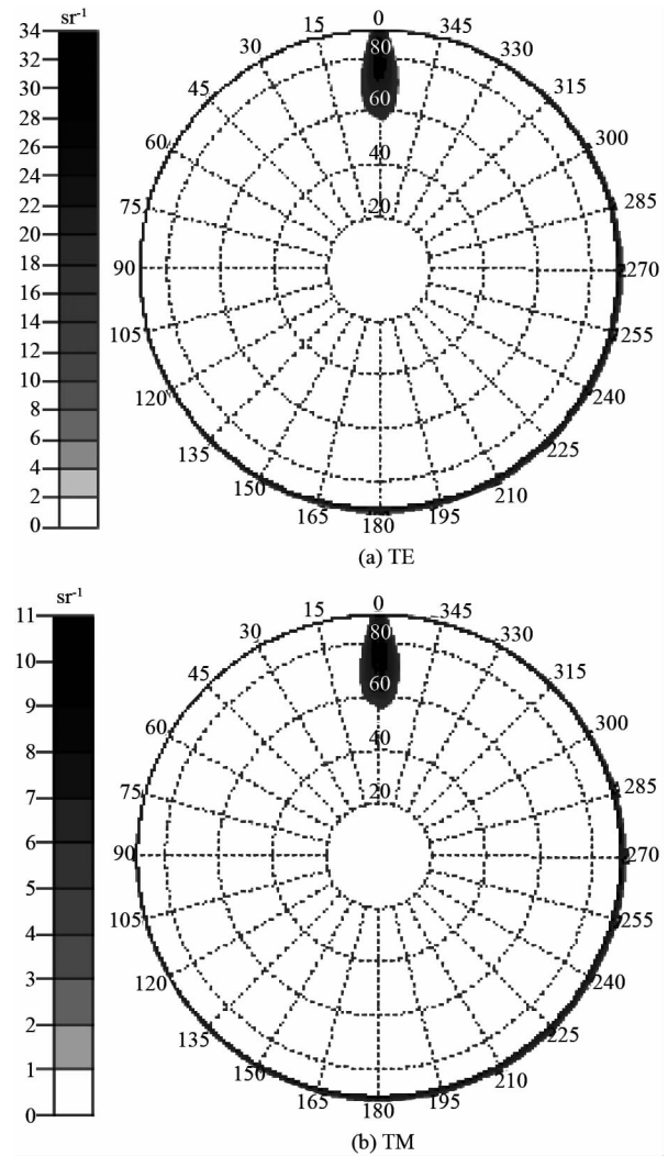
图10 钛合金粗糙表面的 BRDF \cdot \cos\theta_r 极坐标分布图 ( T = 298\text{K}, \theta_i = 80^\circ ) Fig.10 BRDF \cdot \cos\theta_r distribution of rough titanium alloy surface in polar coordinates ( T = 298\text{K}, \theta_i = 80^\circ )
