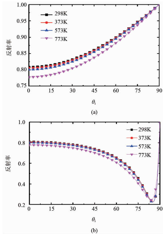
图2 不同温度下光滑钛合金板的反射率(a) TE 波入射, (b) TM 波入射 Fig.2 Reflectivity of smooth titanium alloy plate at different temperature: (a) TE wave incidence, (b) TM wave incidence
