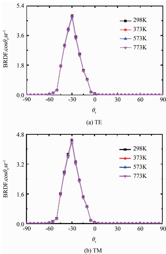
图7 不同温度下钛合金粗糙表面的 BRDF \cdot \cos\theta_r 分布 ( \theta_i = 30^\circ ) Fig. 7 BRDF \cdot \cos\theta_r of rough titanium alloy surface at different temperatures ( \theta_i = 30^\circ )
