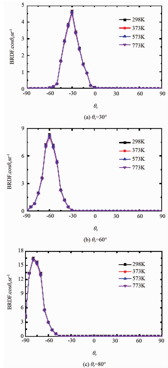
图6 非偏振光入射时不同温度下钛合金粗糙表面的 BRDF \cdot \cos\theta_r 分布 Fig.6 BRDF \cdot \cos\theta_r of rough titanium alloy surface at different temperatures under unpolarized light incidence
