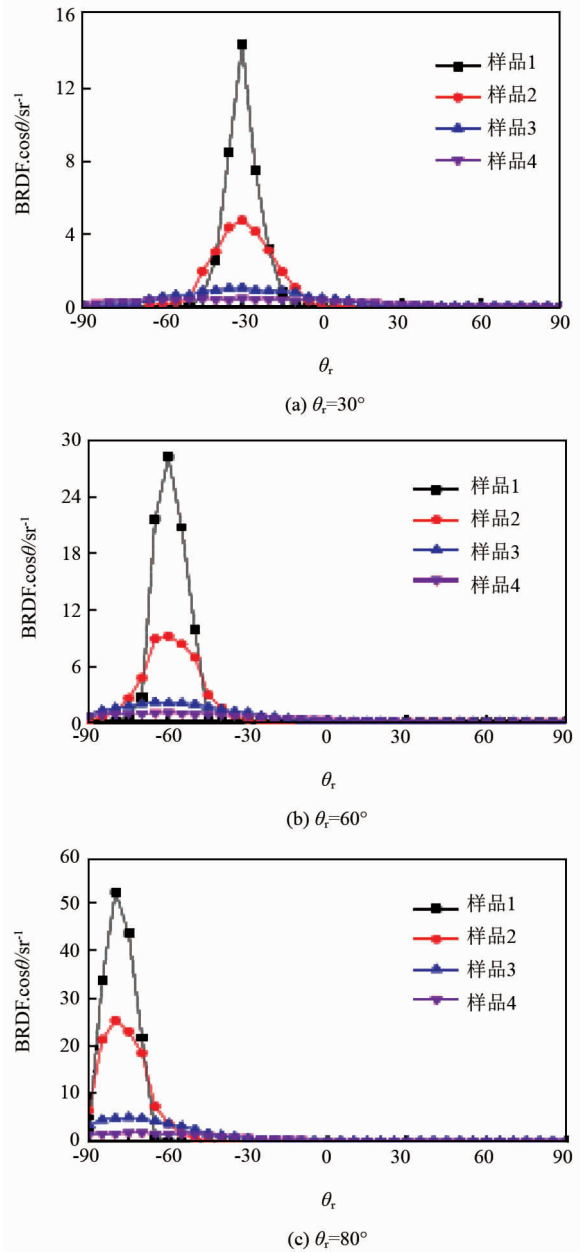
图 4 TE 偏振光入射时不同粗糙度下钛合金的 BRDF \cdot \cos\theta_r of titanium alloy with different surface roughness under TE wave incidence
