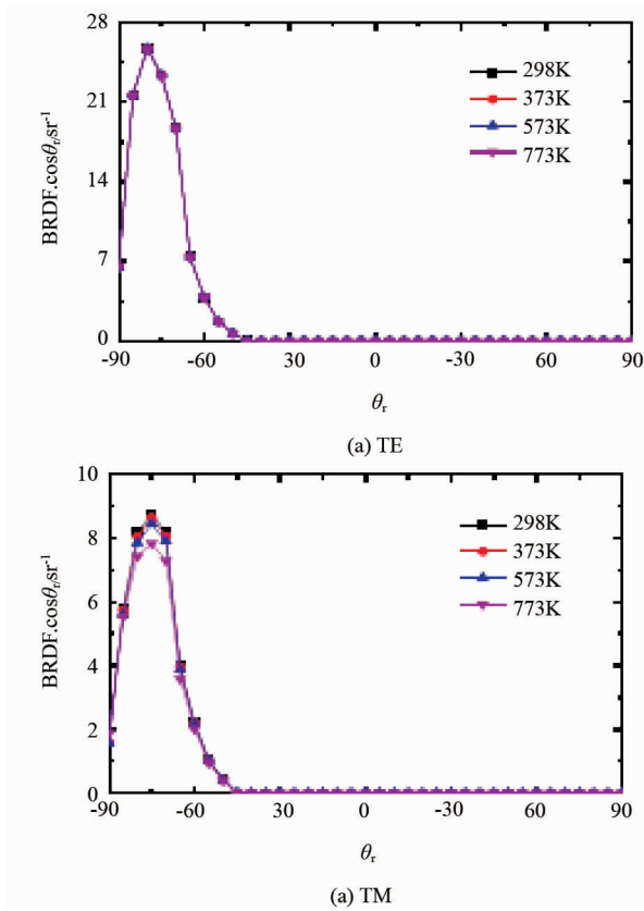
图9 不同温度下钛合金粗糙表面的 BRDF \cdot \cos\theta_r 分布 ( \theta_i = 80^\circ ) Fig.9 BRDF \cdot \cos\theta_r of rough titanium alloy surface at different temperatures ( \theta_i = 80^\circ )
