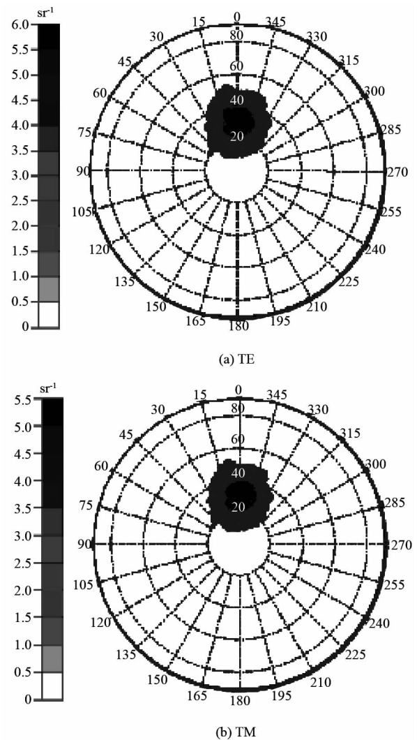
图8 钛合金粗糙表面的 BRDF \cdot \cos\theta_r 极坐标分布图 ( T = 298 \text{ K}, \theta_i = 30^\circ ) Fig. 8 BRDF \cdot \cos\theta_r distribution of rough titanium alloy surface in polar coordinates ( T = 298 \text{ K}, \theta_i = 30^\circ )
