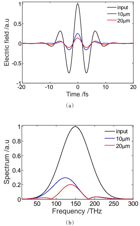
Fig. 3 The pulse distortions of few-cycle laser pulse with a wavelength of 2 μm induced by the EOS with different thicknesses: (a) shows the time waveforms and (b) shows their frequency spectra, respectively
