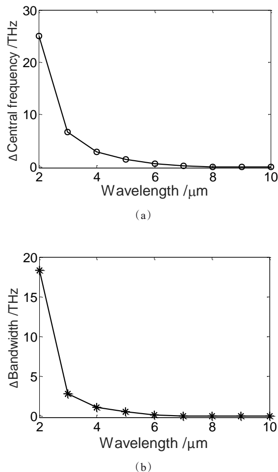
Fig. 5 The changing of (a) the central frequency and (b) the bandwidth depending on the wavelength of the few-cycle laser pulse from 2 \mu\text{m} to 10 \mu\text{m}
