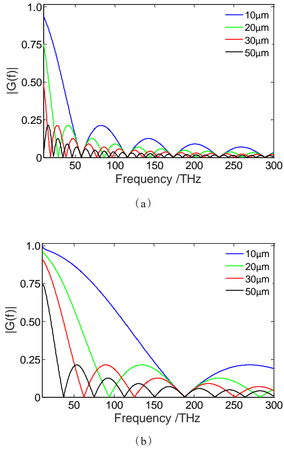
Fig. 2 The response function of the EOS with different GaSe thicknesses (10 μm, 20 μm, 30 μm, and 50 μm) with two different probe laser wavelengths: (a) is with 800 nm and (b) is with 1030 nm
