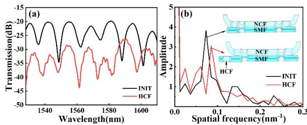
Fig. 8 (a) A comparison of the transmission spectra of the MTP-MZI without and with HCF; (b) The corresponding spatial frequency spectra
