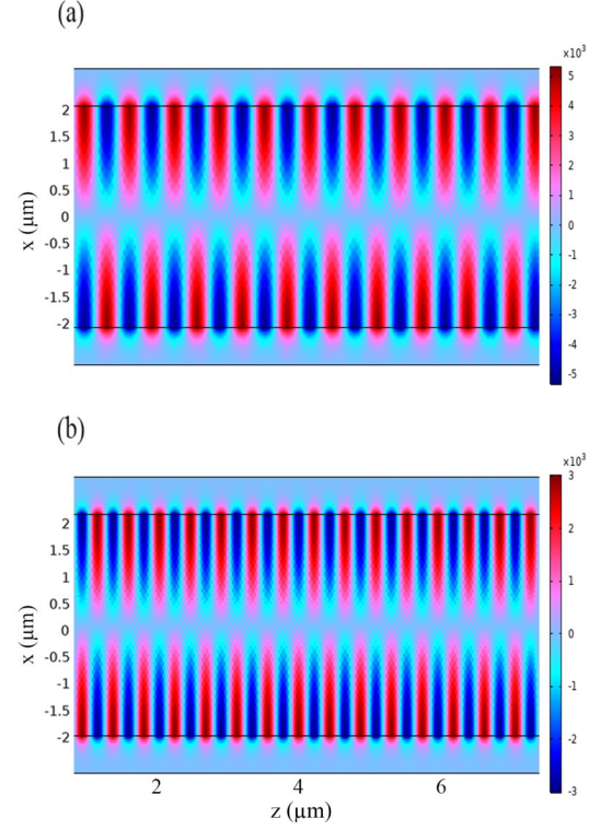
Fig. 7 The variations in the x -component of the electric field of THz radiation in the 2D cross-section of the GaAs waveguide for various in-plane modes
