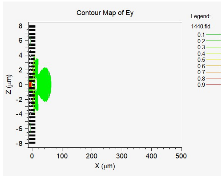
Fig. 7 Simulation of the light-emitting beaming of 1.440\mu\text{m}
