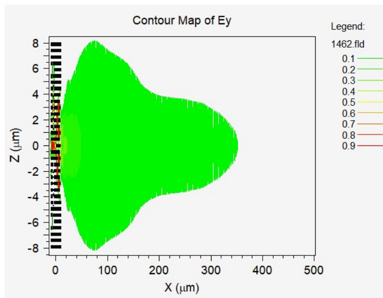
Fig. 8 Simulation of the light-emitting beaming of 1.462\mu\text{m}
