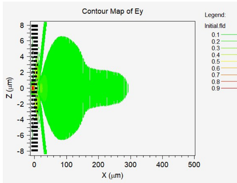
Fig. 3 Simulation of the initial model of the light-emitting beaming
