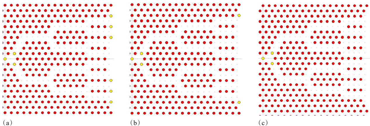
图5 调整后的出射端结构 a)6个介质柱 b)2个介质柱 c)0个介质柱:a)6 medium columns b)2 medium columns c)0 medium columns Fig. 5 The structure of the emitting end after adjustment
