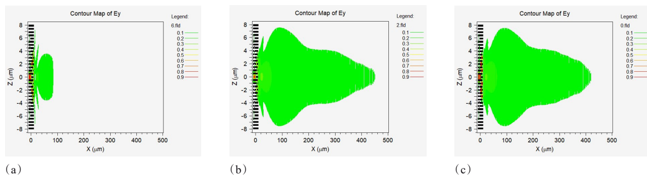
图6 优化后结构的出射光集束仿真 a)6个介质柱 b)2个介质柱 c)0个介质柱:a)6 medium columns b)2 medium columns c)0 medium columns Fig. 6 Simulation of the light-emitting beaming of the optimized structure
