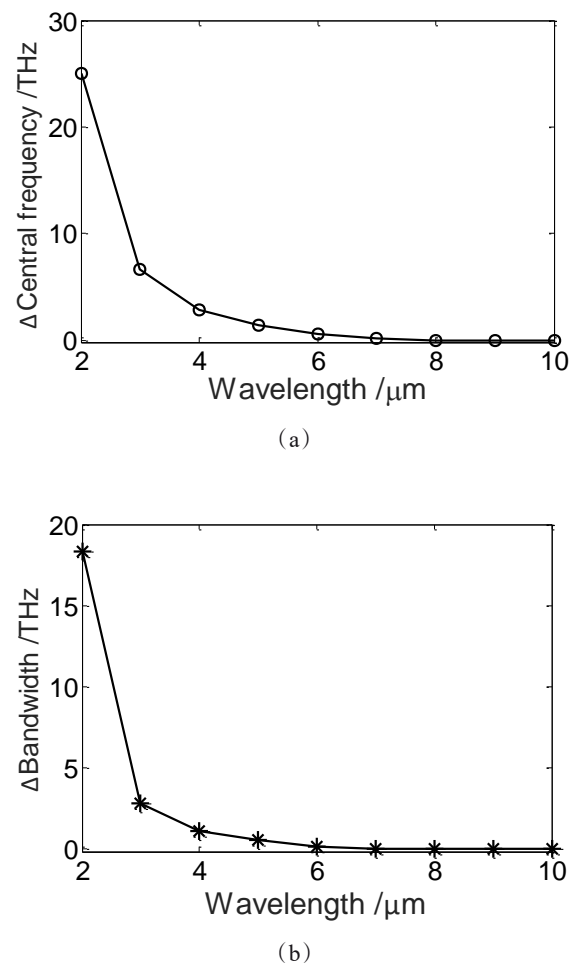
Fig. 5 The changing of (a) the central frequency and (b) the bandwidth depending on the wavelength of the few-cycle laser pulse from 2 \mu\text{m} to 10 \mu\text{m}
