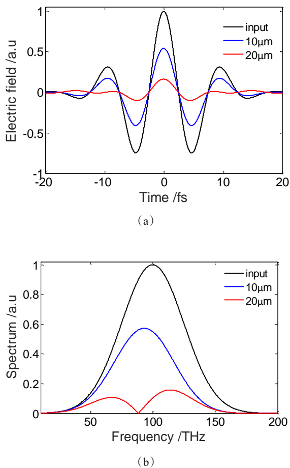
Fig. 4 The pulse distortions of few-cycle laser pulse with a wavelength of 3 \mu\text{m} induced by the EOS with different thicknesses: (a) shows the time waveforms and (b) shows their frequency spectra
