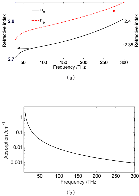
Fig. 1 (a) The ordinary and extraordinary light refractive indexes and (b) the absorption of GaSe crystal in the mid-infrared range 图1 寻常光和非寻常光在硒化镓晶体中的(a)折射率和(b)吸收系数
