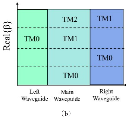
Fig. 1 Schematic structure of the MRW device structure and principle: (a) Cross-section of the MRW; (b) Design principle of mode coupling 图1 MRW 器件结构和原理示意图:(a) 器件横截面;(b) 主波导与左、右辅助波导的模式耦合设计原则
