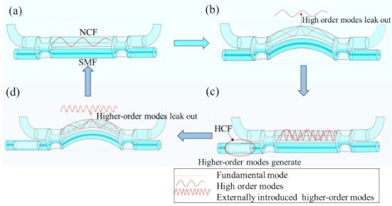
Fig. 5 Flow chart of MTP-MZI model monitoring experiment. : (a) Initial state of the mode monitor; (b) Mode characterization experiments with MTP-MZI bending; (c) Introduction of higher-order modes; (d) Experimental validation of mode monitoring 图5 MTP-MZI模式监测实验流程图。(a)模式监测器初始状态;(b)模式监测器特性;(c)引入高阶模式;(d)实验验证模式监测
