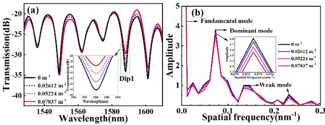
Fig. 6 (a) The transmission spectra of MTP-MZI with variation curvatures; (b) The corresponding spatial frequency spectrum 图6 (a)不同曲率MTP-MZI的透射光谱;(b)相应的空间频谱
