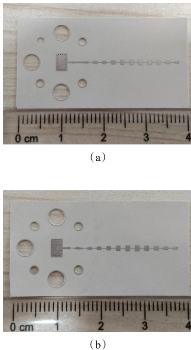
Fig. 10 Prototype of millimeter wave radar antenna: (a) gradient; (b) wavy
